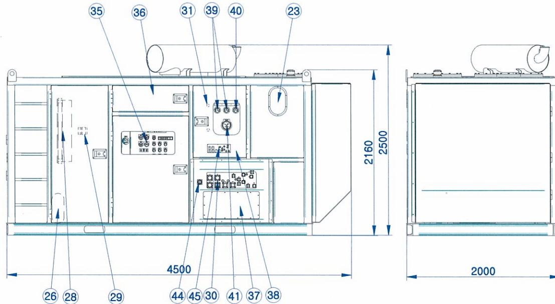
VIEW A
